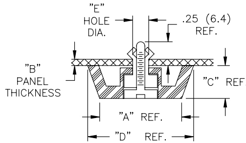
WITH DRIVE SCREW
