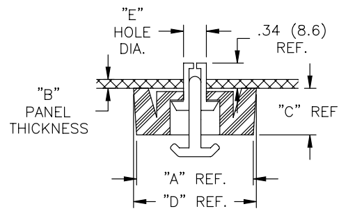
WITH PUSH RIVET
